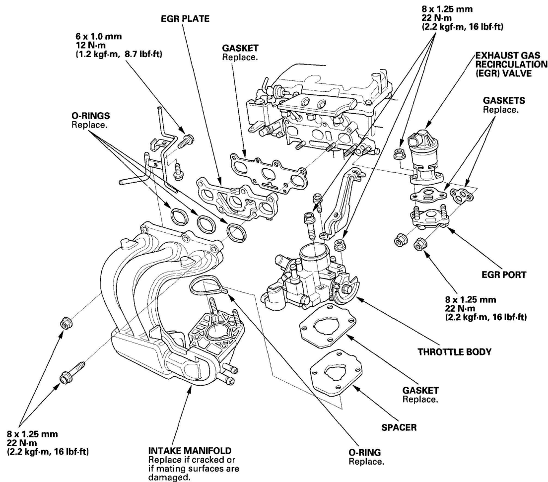
Fig. 1: Exploded View Of Intake Manifold Courtesy of AMERICAN HONDA MOTOR CO., INC.
