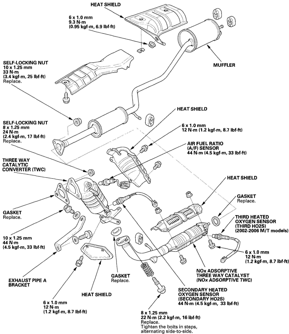
Fig. 2: Exploded View Of Exhaust Pipe And Muffler Courtesy of AMERICAN HONDA MOTOR CO., INC.
