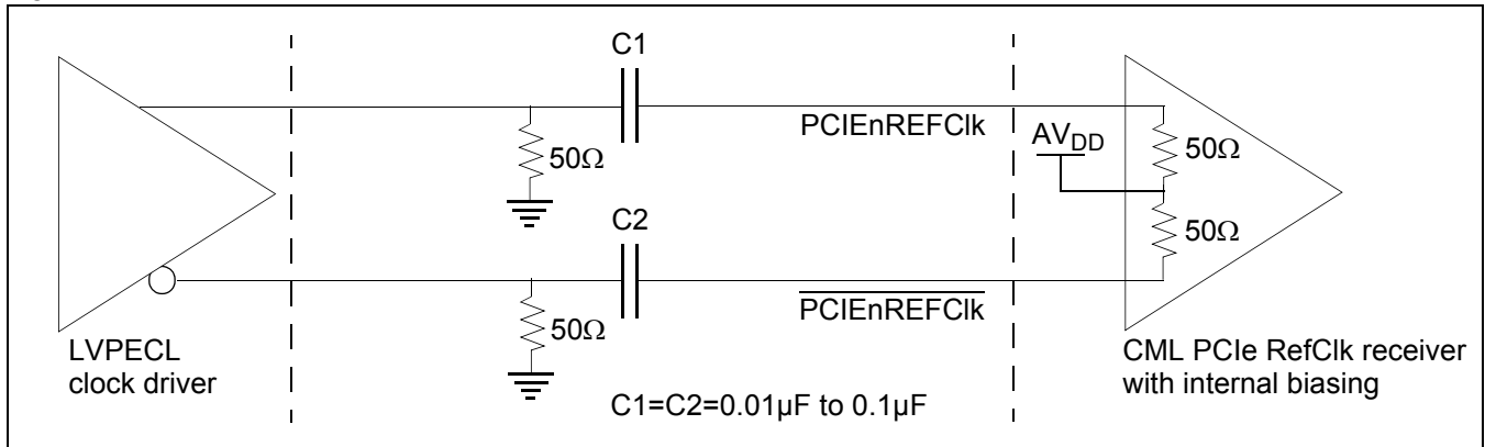
Figure 12. LVPECL PCIe Reference Clock
