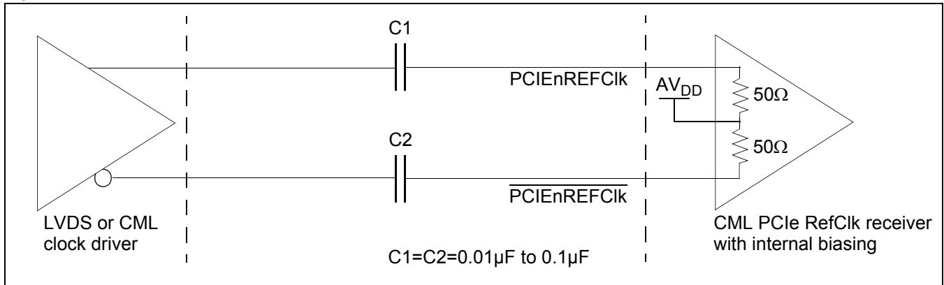
Figure 11. LVDS or CML PCIe Reference Clock
