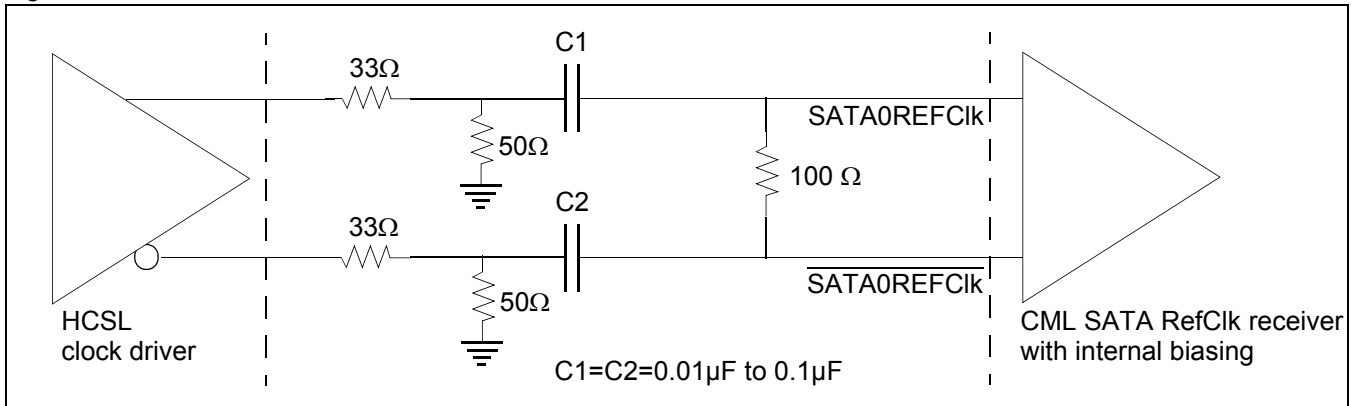
Figure 16. HCSL SATA Reference Clock
