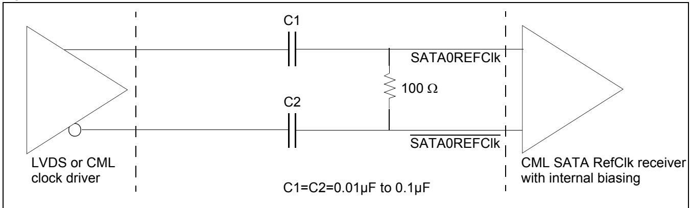
Figure 14. LVDS or CML SATA Reference Clock
