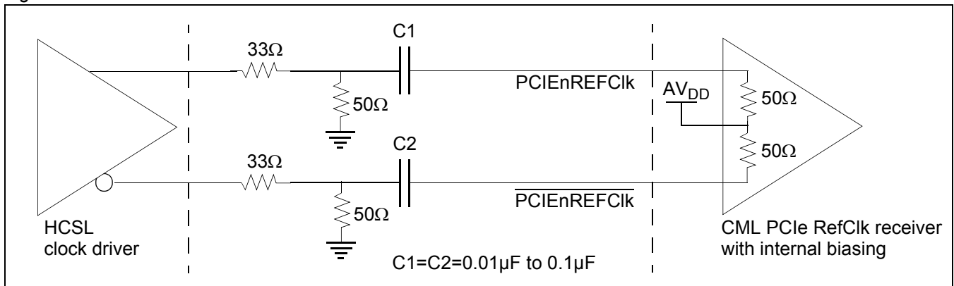
Figure 13. HCSL PCIe Reference Clock
