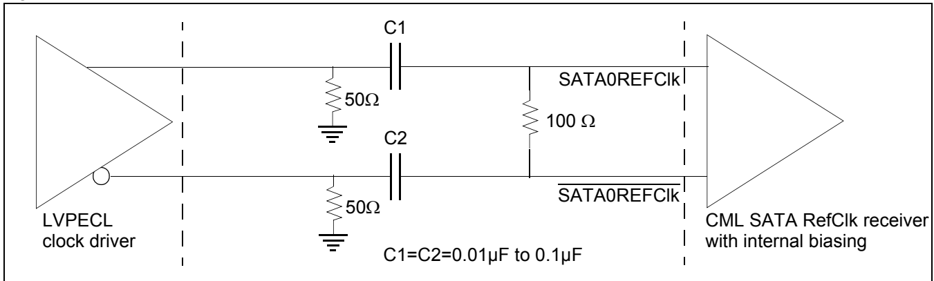
Figure 15. LVPECL SATA Reference Clock
