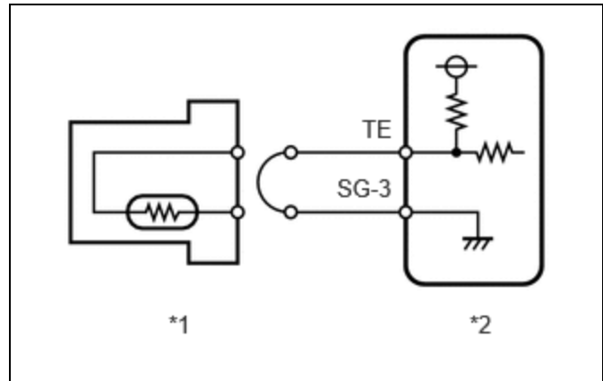
*1 Evaporator Temp. Sensor (No. 1 Cooler Thermistor) *2 Air Conditioning Amplifier Assembly
